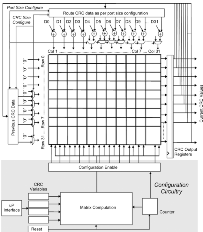
Fig.1 Field programmable CRC architecture.
