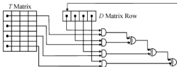
Fig.2. Programmable CRC array cell.
