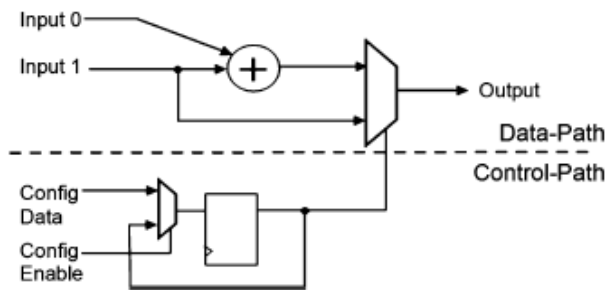
Fig.2. Programmable CRC array cell.
