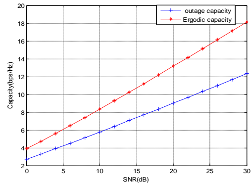
Fig (11) Comparison of Ergodic and Outage Capacities with CSI at receiver
