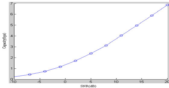
Fig (6) Capacity Vs SNR for N_t = 1 and N_r = 1
