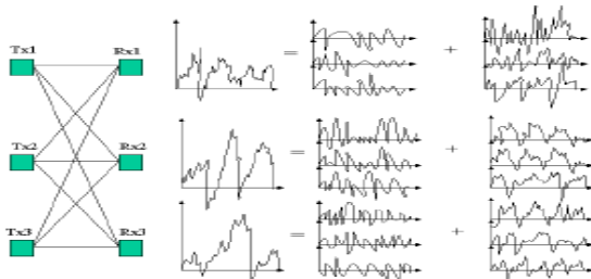
Fig 2 Separation of the received signal into intelligible and non-intelligible components, i.e. signal and noise.
