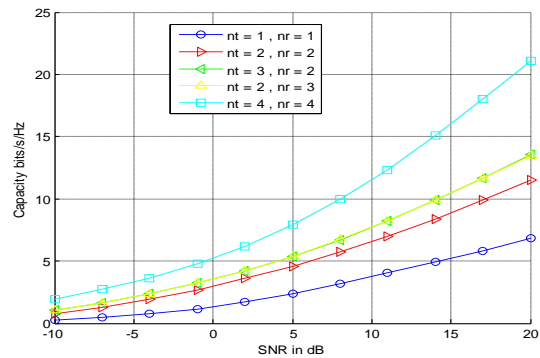
Fig (9) Capacity Vs SNR for N_t = 4 and N_r = 4
