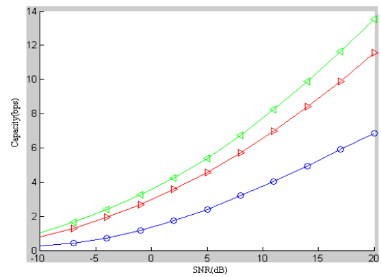
Fig (8) Capacity Vs SNR for N_t = 3 and N_r = 2
