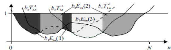
Fig (4) Multi-User Water filling algorithm.
